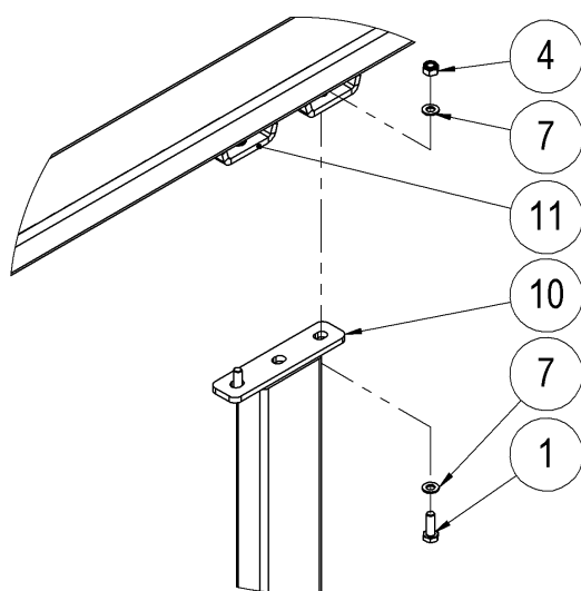
DETAIL B
