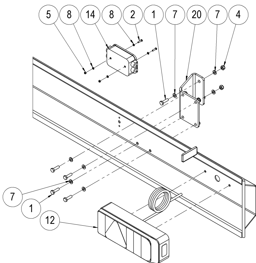
DETAIL A
