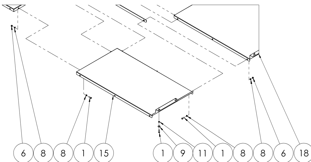
DETAIL C
