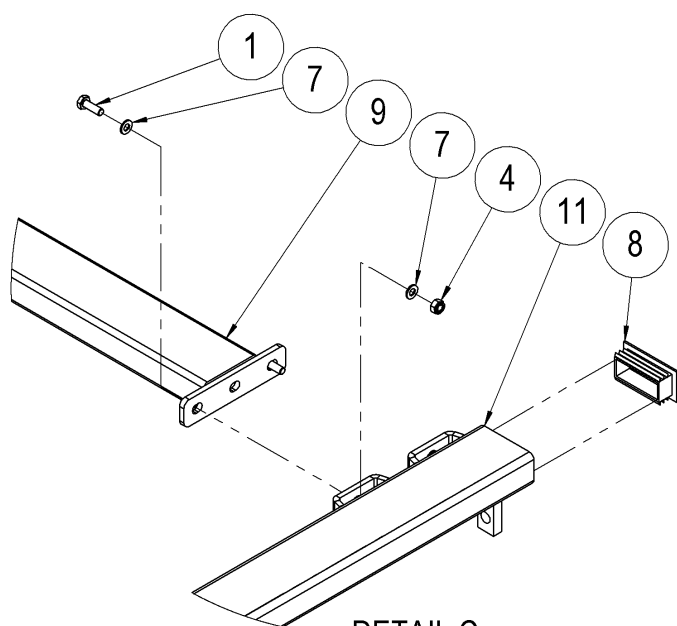
DETAIL C
